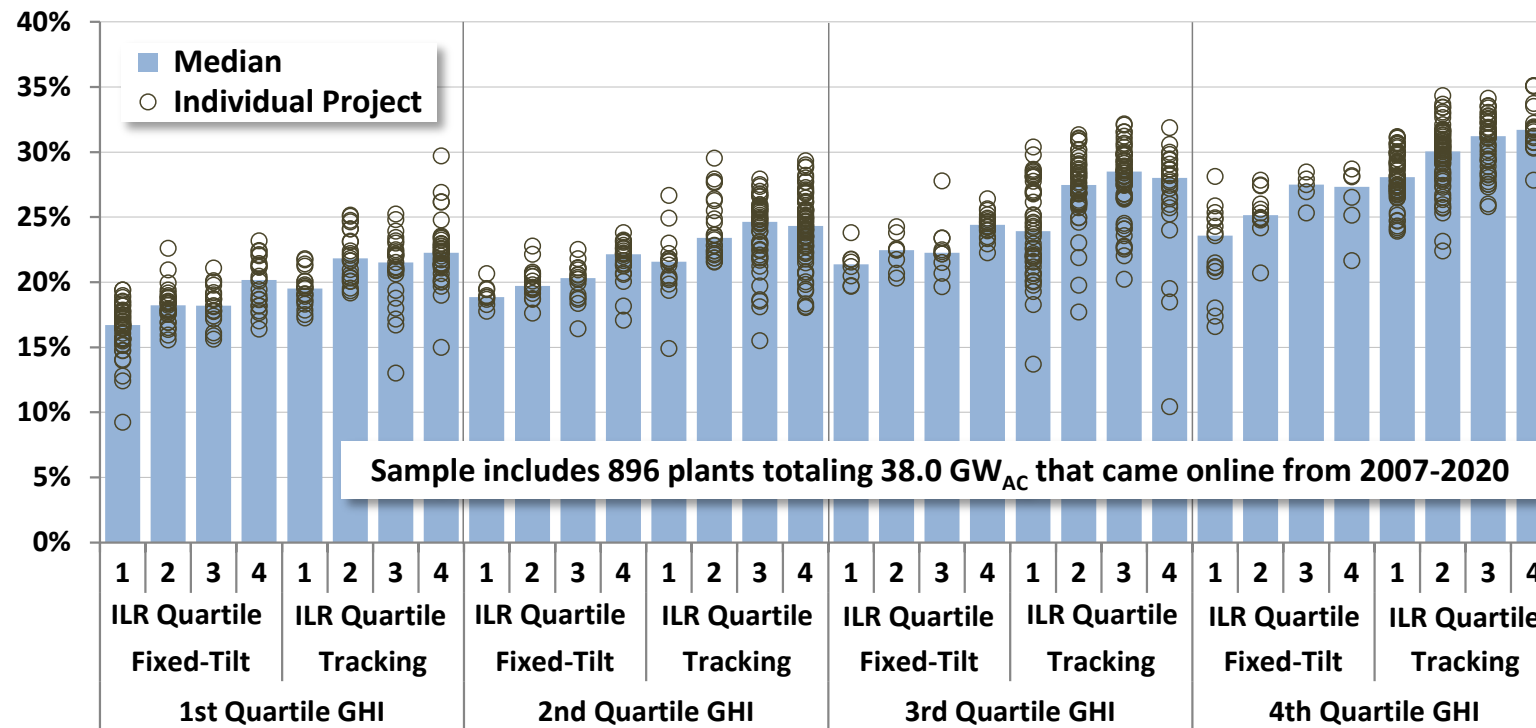
Cumulative AC Capacity Factor
