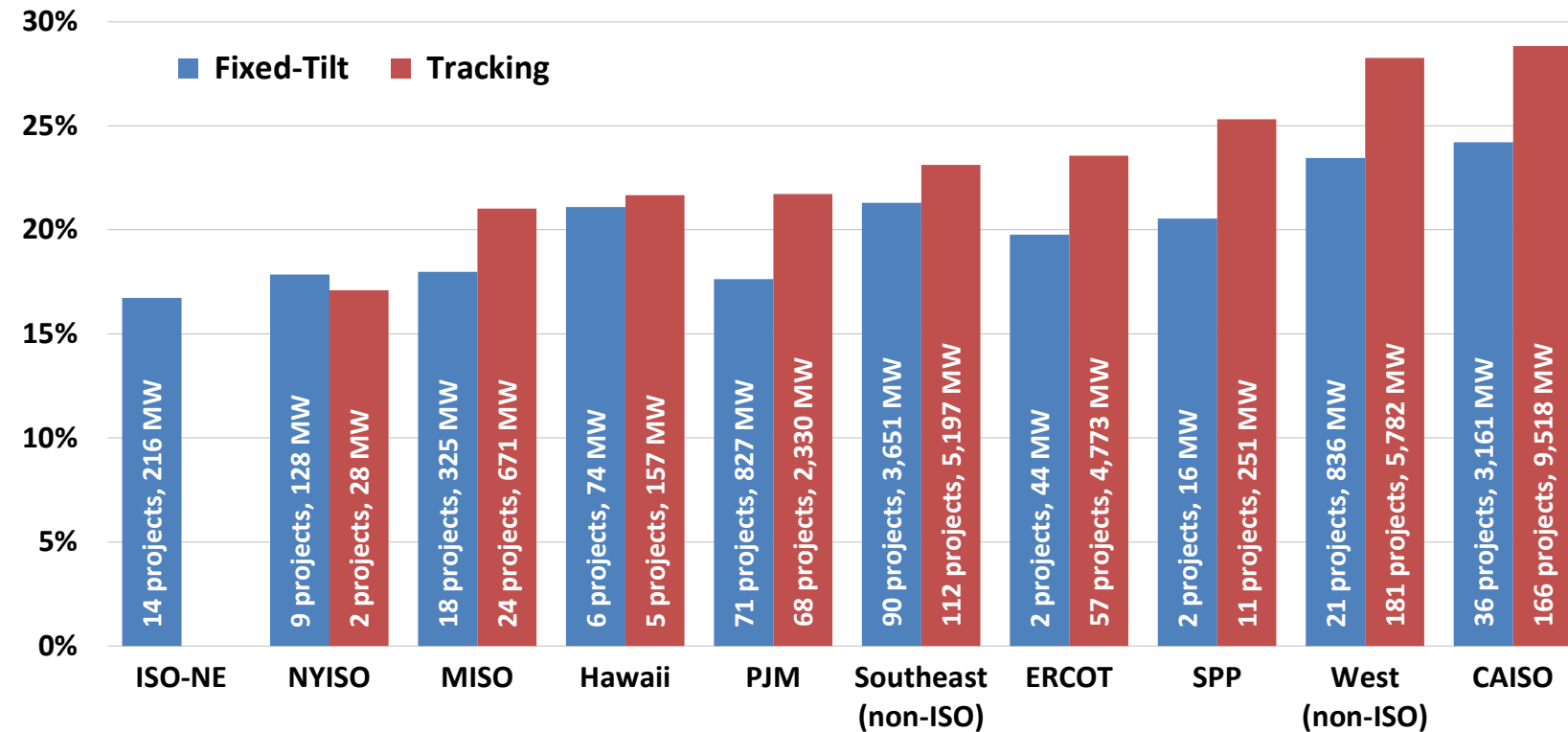
Average Cumulative AC Capacity Factor
