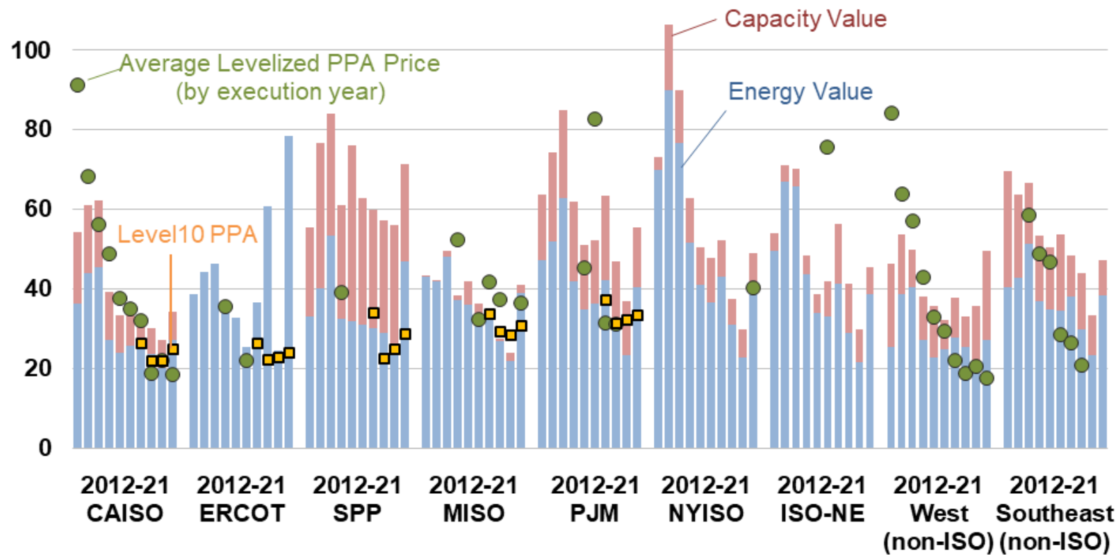
Solar Value and PPA Price (2021 $/MWh)
