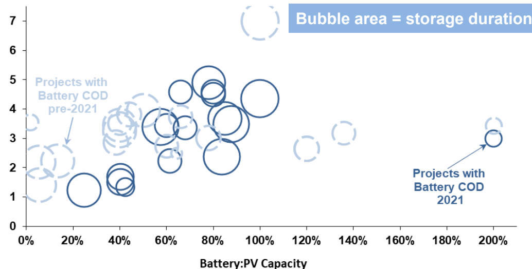
Combined PV+Battery Costs (2021 $/W AC -PV)
