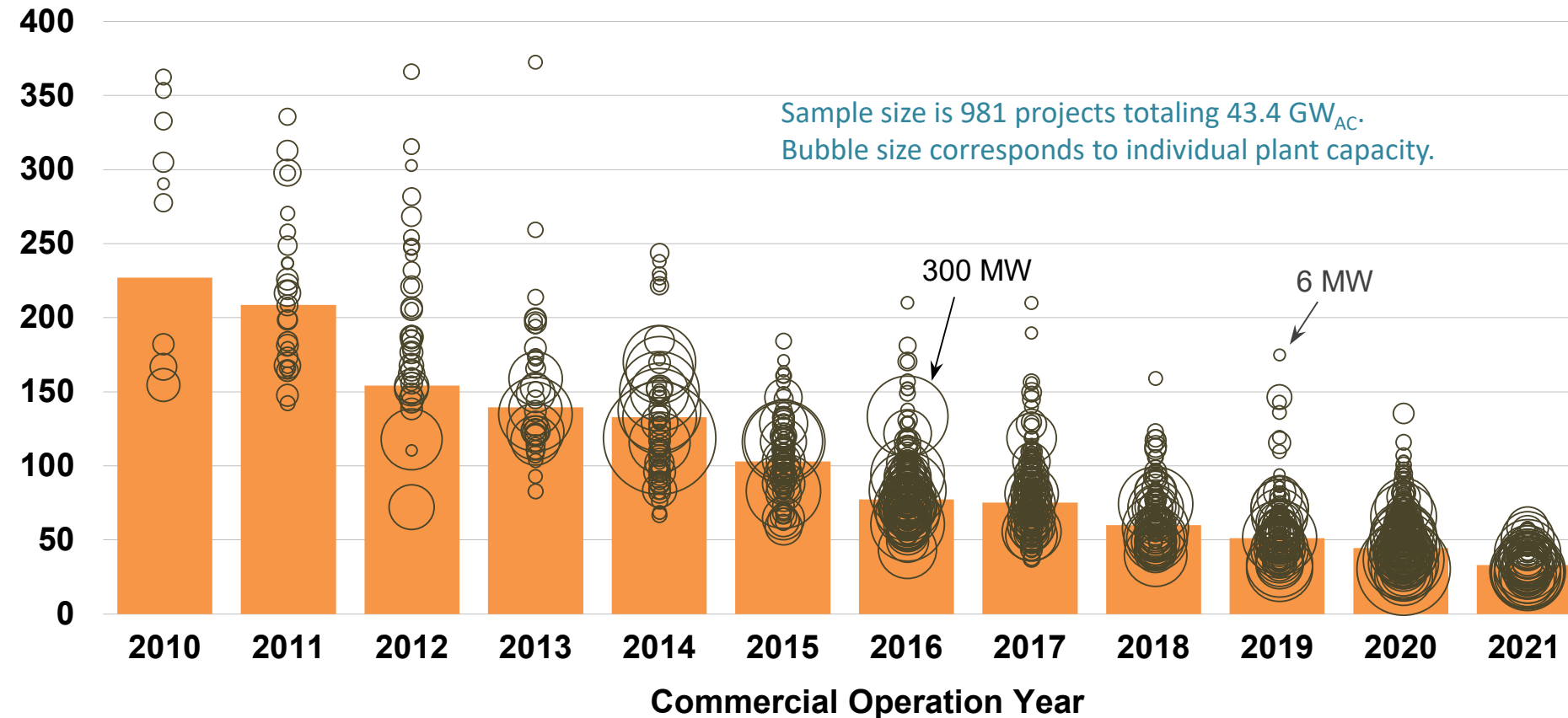
Generation-Weighted Average and Project-Level LCOE (2021 $/MWh)
