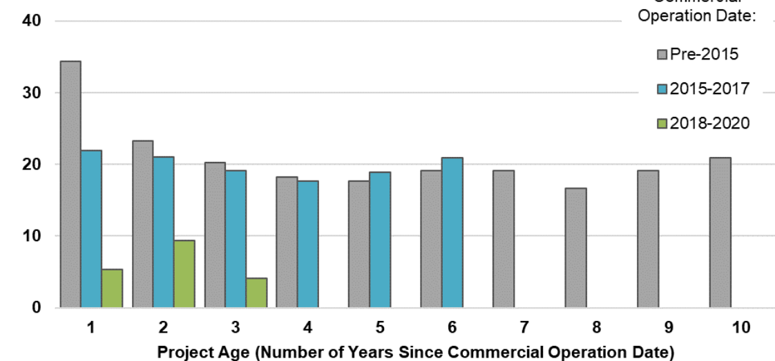
Median O&M Cost (2021 $/kW AC -year)
