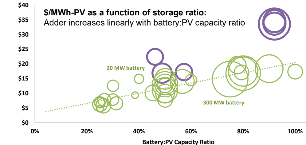
Levelized Storage Adder (2021 $/MWh-PV)
