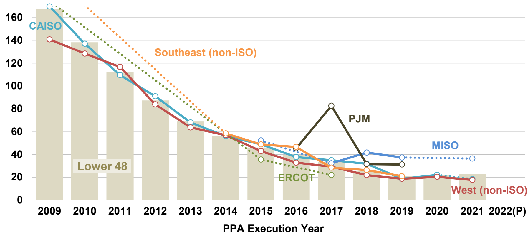
Average Levelized PPA Price (2021 $/MWh)
