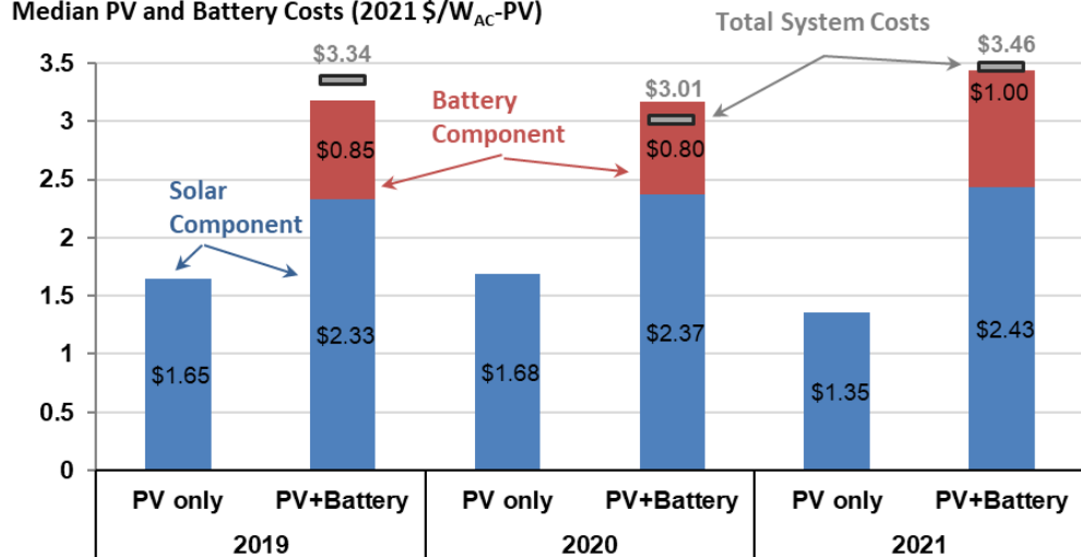
Median PV and Battery Costs (2021 $/W AC -PV)
