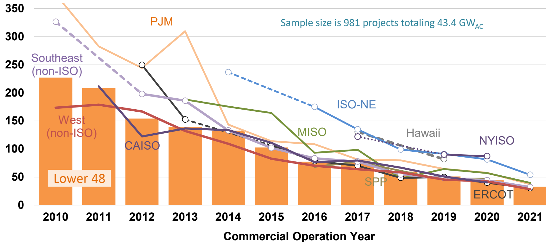
Generation-Weighted Average LCOE (2021 $/MWh)
