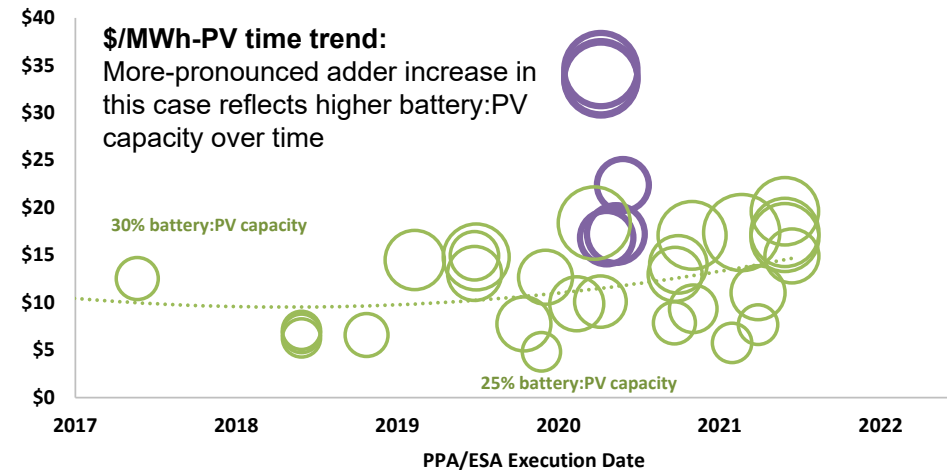
Levelized Storage Adder (2021 $/MWh-PV)
