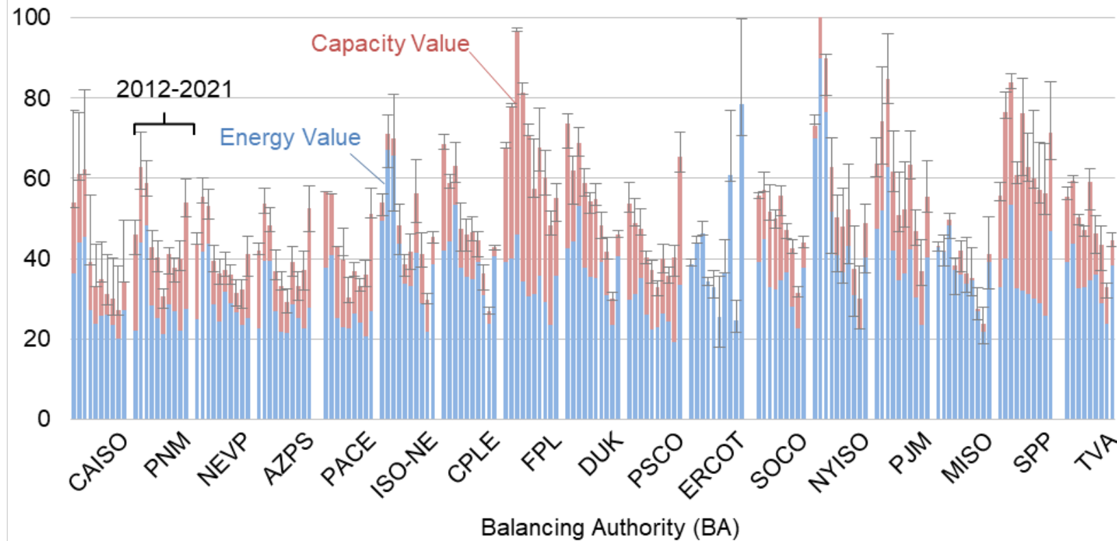
Average Solar Value, with 10 th /90 th Percentiles of Combined Value (2021 $/MWh)
